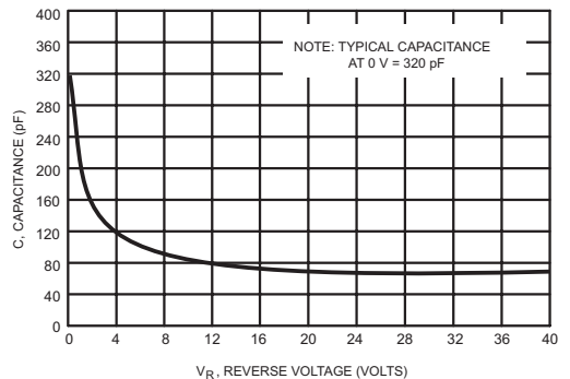
FIG.6- TYPICAL CAPACITANCE
