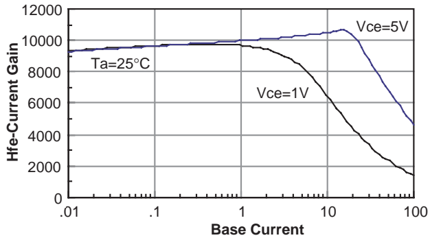
Figure 5. Hfe current gain versus base current
