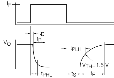
Figure 9. Switching schematic
