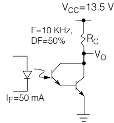
Figure 9. Switching schematic
